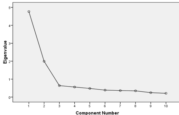
Scree Plot
